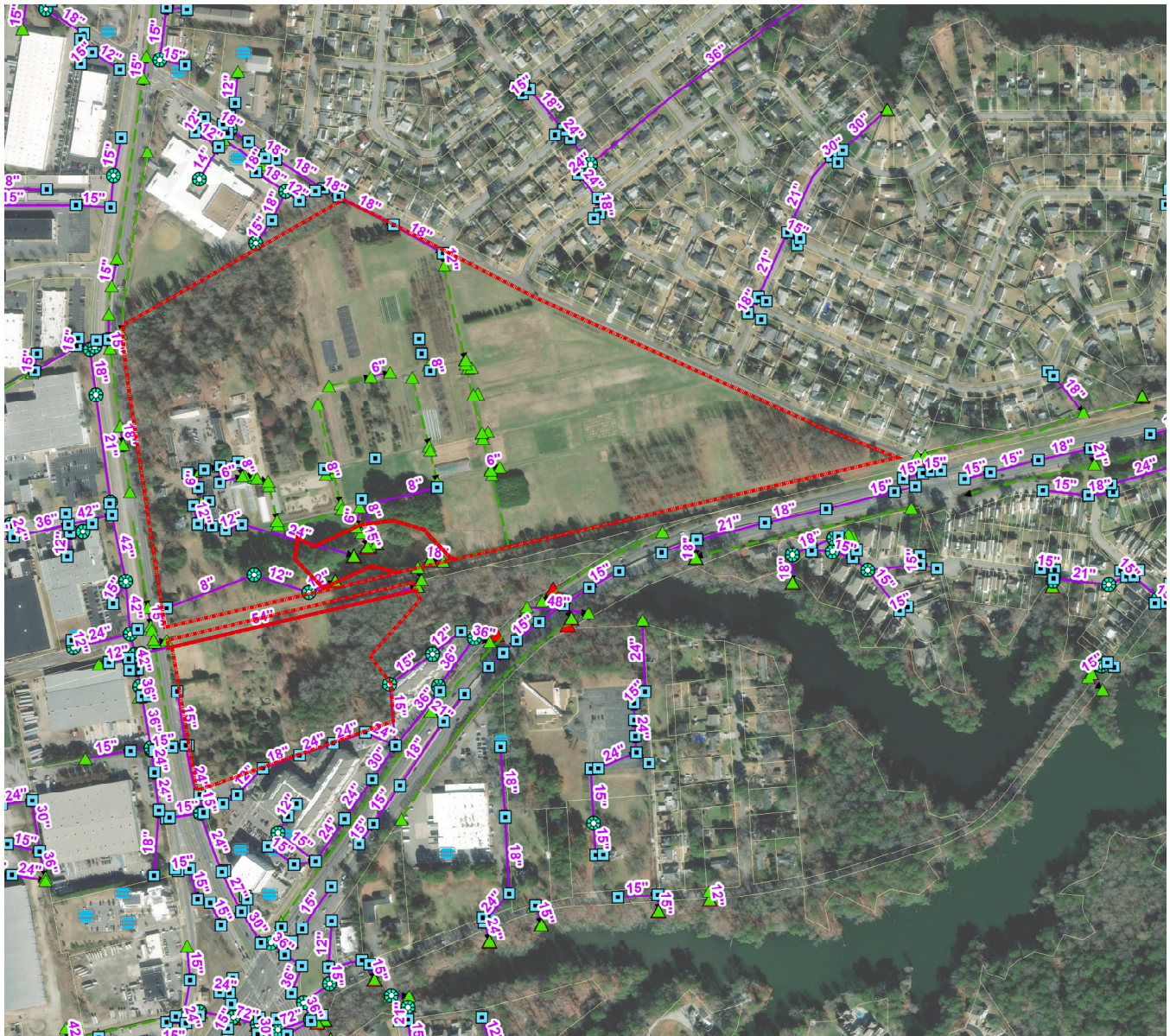
Figure 19. Existing Site - Stormwater Utilities Map
