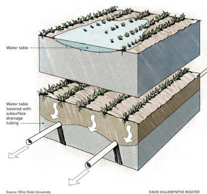
Figure 40. Tile Drainage Impact. Tile drainage lowers the water table, protecting roots from extended exposure to wet soil. Image credit: Ohio State University and David Kallemyn - The Register.
